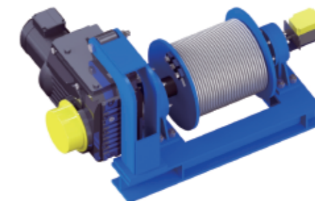
Construction Winch
